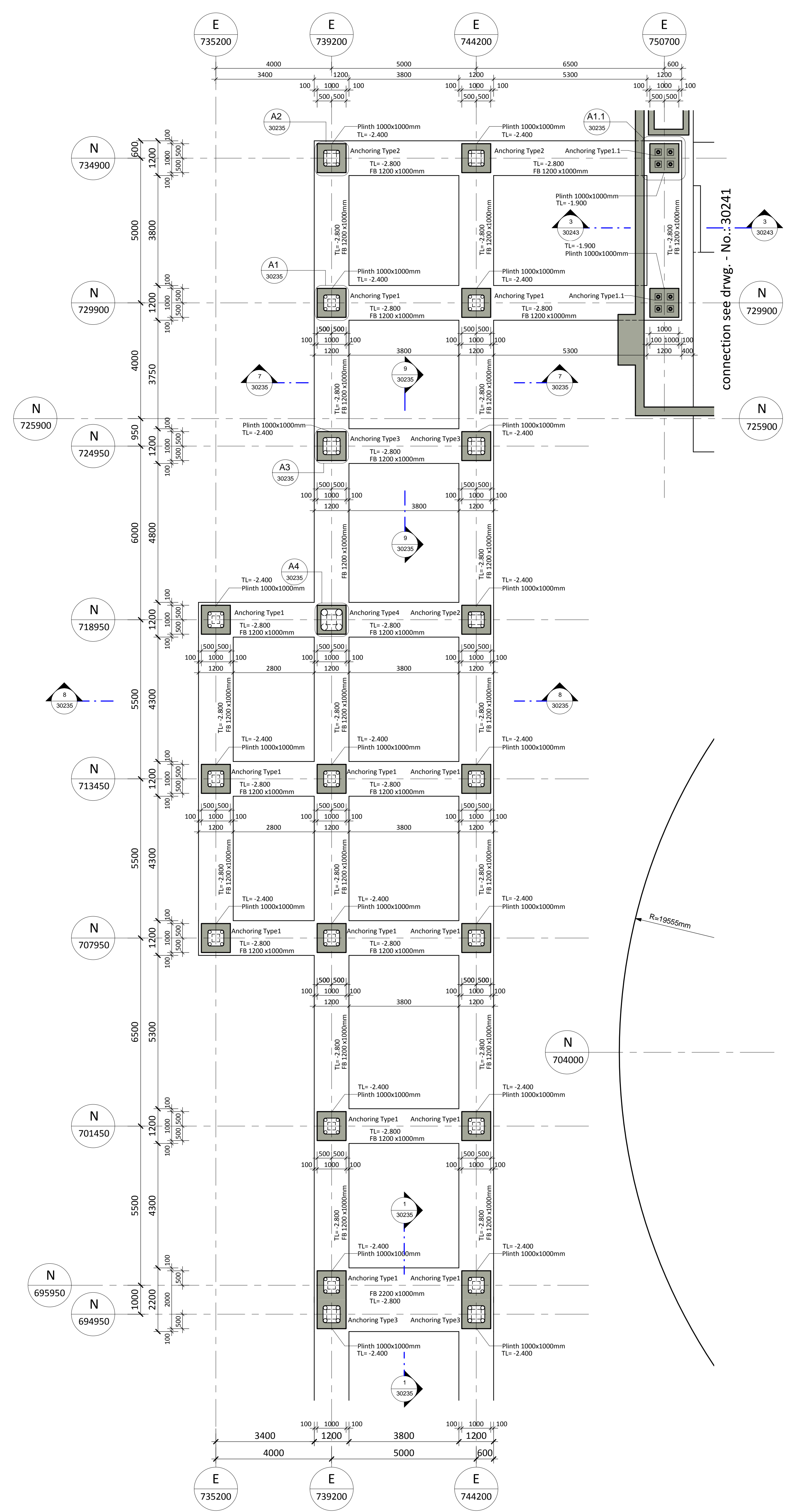
1 PLAN VIEW - FOUNDATIONS PIPE RACK - PART 1 1 : 75
